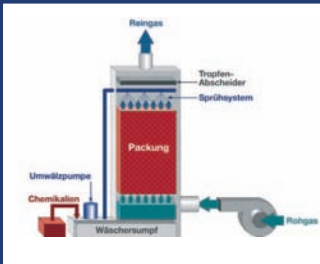
Air treatment
